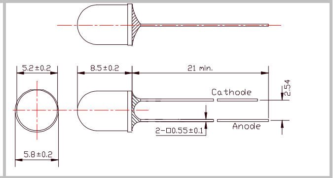
Figure 4 Ø5 mold (type 04)
