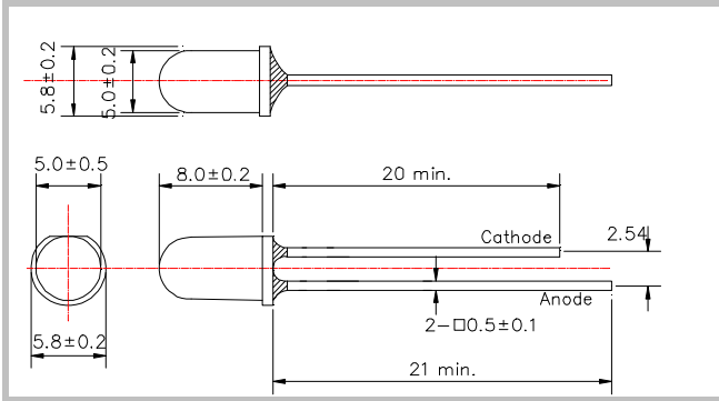
Figure 3 Ø5 mold (type 03)
