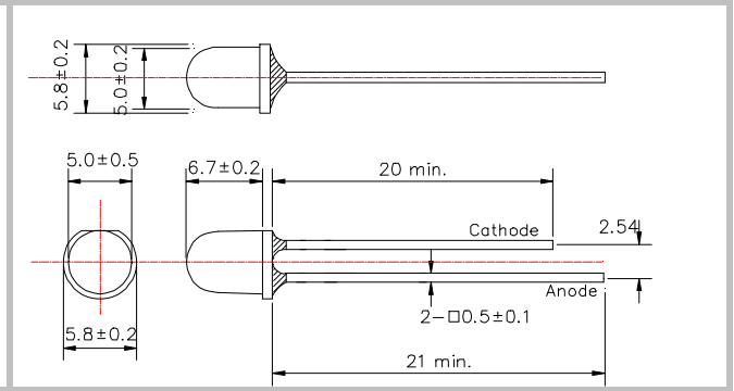
Figure 6 Ø5 mold (type 06)
