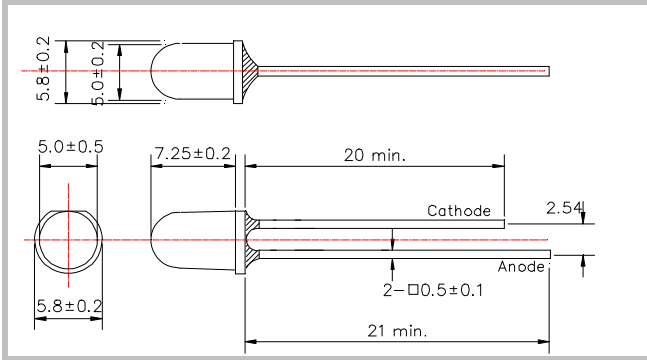
Figure 5 Ø5 mold (type 05)
