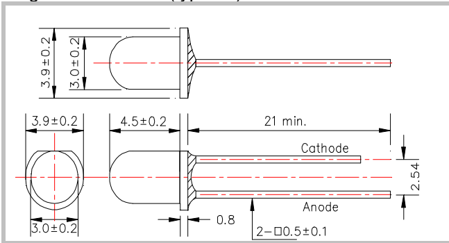
Figure 9 Ø3 mold (type 33)
