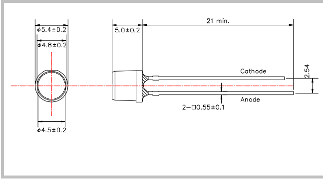
Figure 7 Ø5 mold (type 09)
